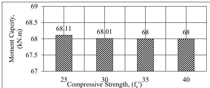
Figure 7. Effect of concrete strength on moment capacity
